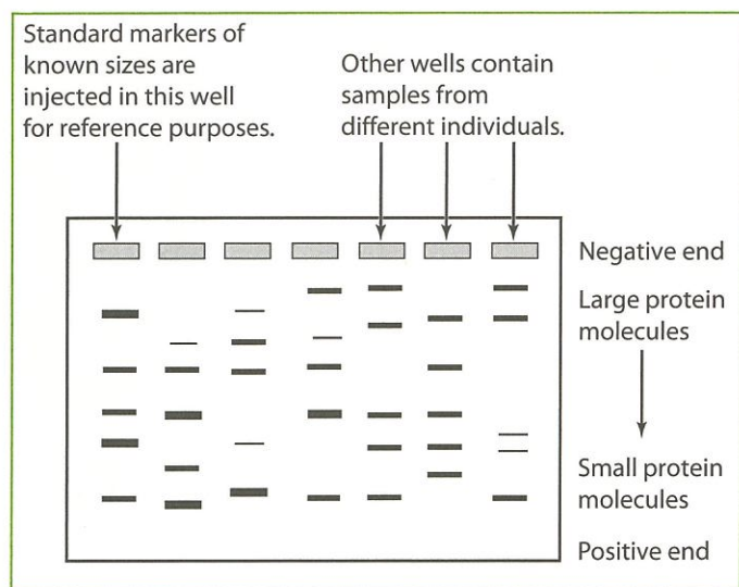
Figure 9-18. Protein gel electrophoresis: Protein gels are typically run vertically, with the gel block standing on end.
