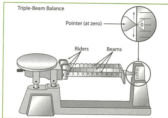
Figure 9-6. Triple-beam balance
